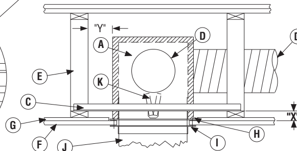
END VIEW W/DUCT (556RD, 556RDD)
