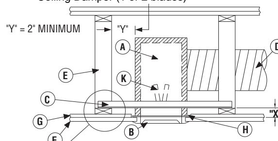
END VIEW W/GRILLE (556RD, 556RDD)
