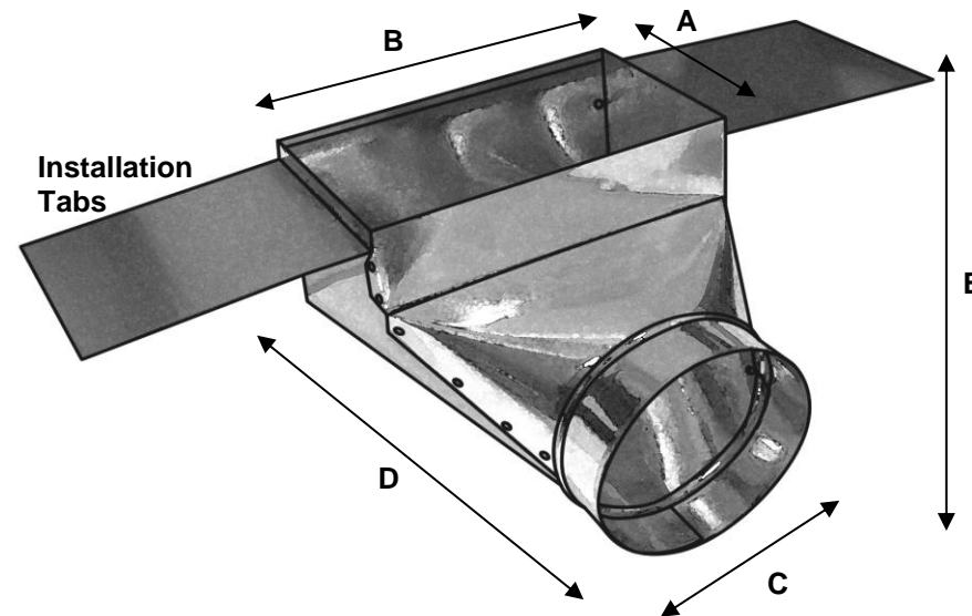
Model 243B 90DEG Register Boot
